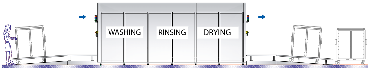
Multi-chamber system in floor-level installation
