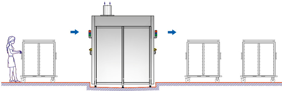
Single-chamber system in pit installation
